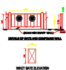
WICKET GATE ELEVATION
