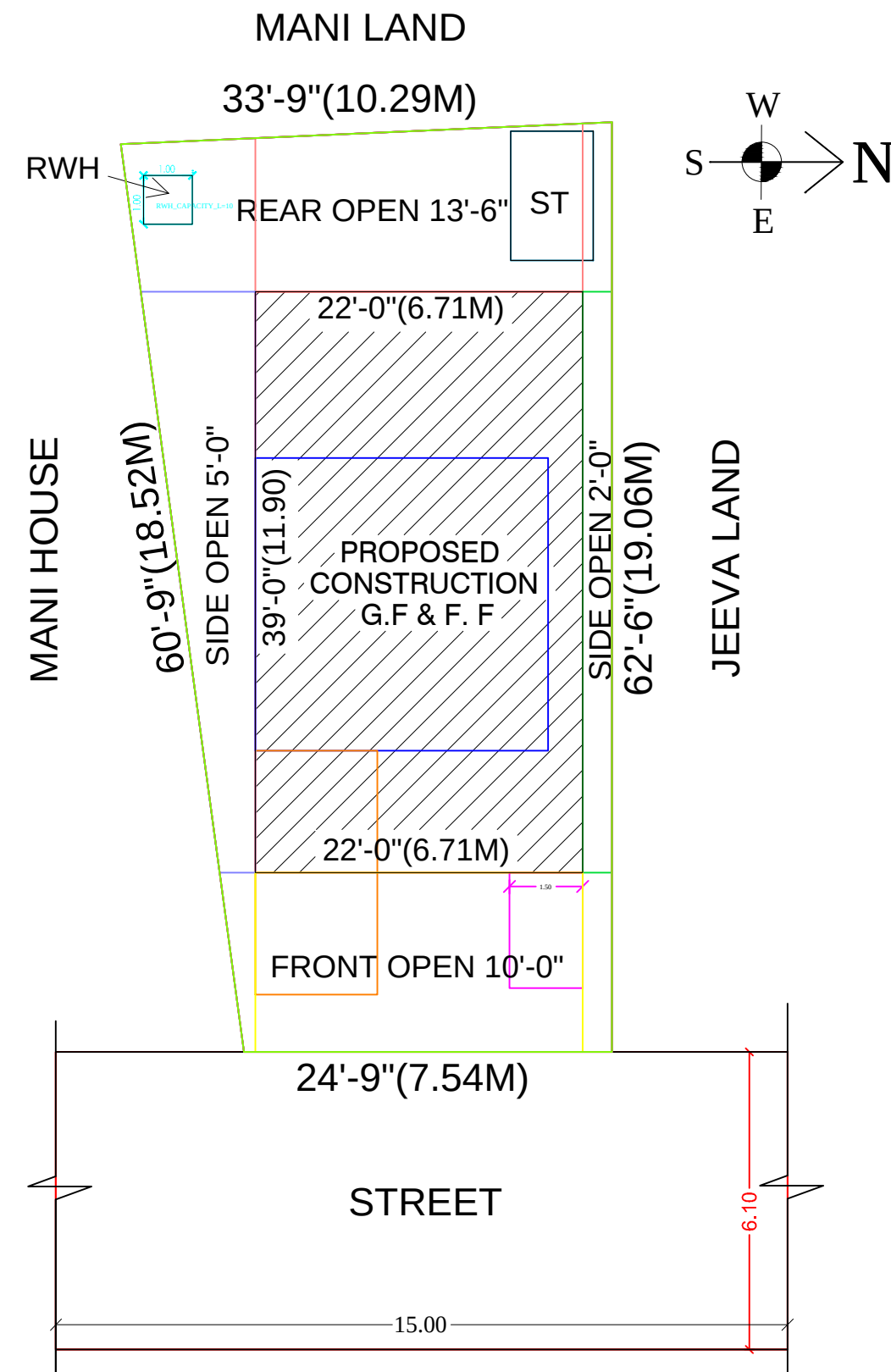
SITE PLAN SCALE: 1CM: 1M
