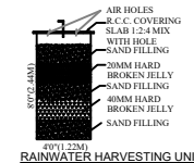
RAINWATER HARVESTING UNIT (NOT TO SCALE)
