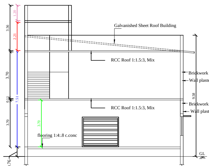
SECTION ON JJ (SCALE: 1CM : 1M)
