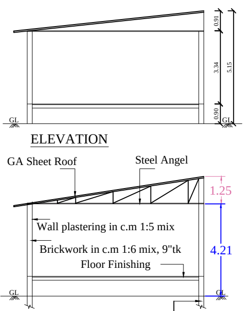
SECTION NN (SCALE: 1CM : 1M)
