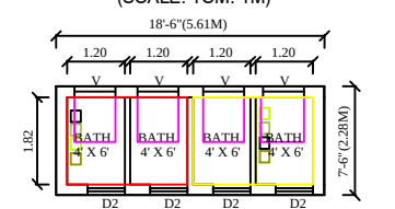
TOILET BLOCK PLAN
