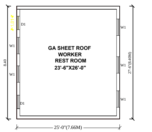
WORKERS REST ROOM PLAN
