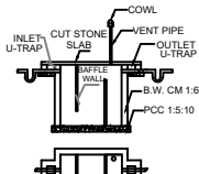
SEPTIC TANK DETAILS SIZE :6'0" x 3'0" x 6'0"
