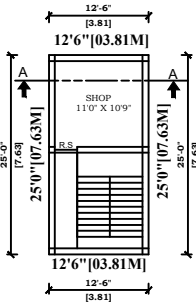
PRO.FIRST FLOOR PLAN.
