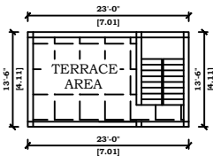
TERRACE FLOOR
