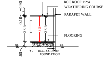
SECTION ON ' AA '
