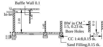
SEPTIC TANK & SOAK PIT
