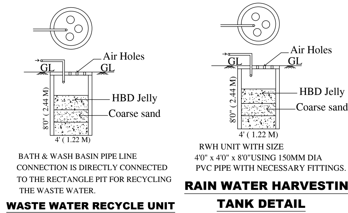
WASTE WATER RECYCLE UNIT
