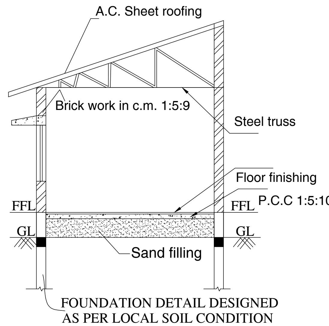
SECTION ON "JS"
