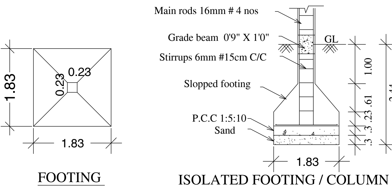
COLUMN DETAIL
