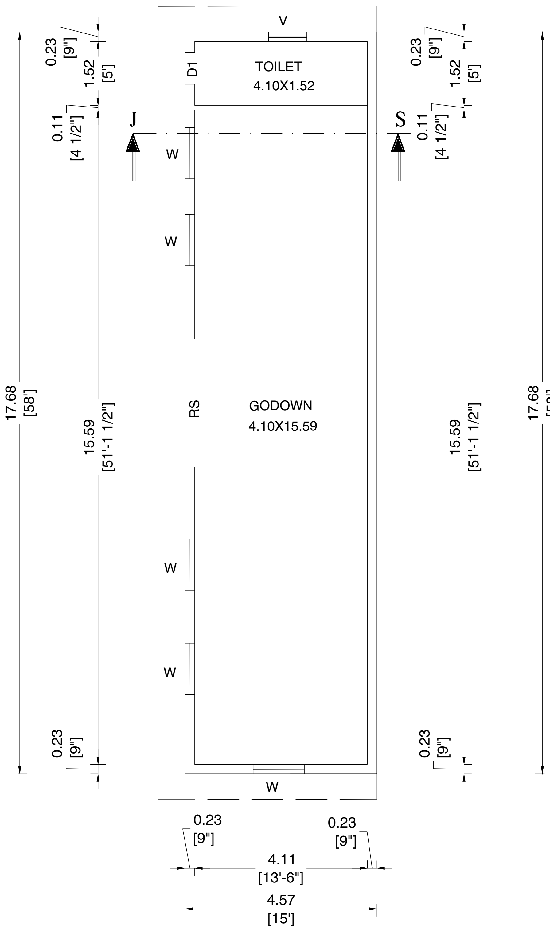
PRO.GROUND FLOOR PLAN
