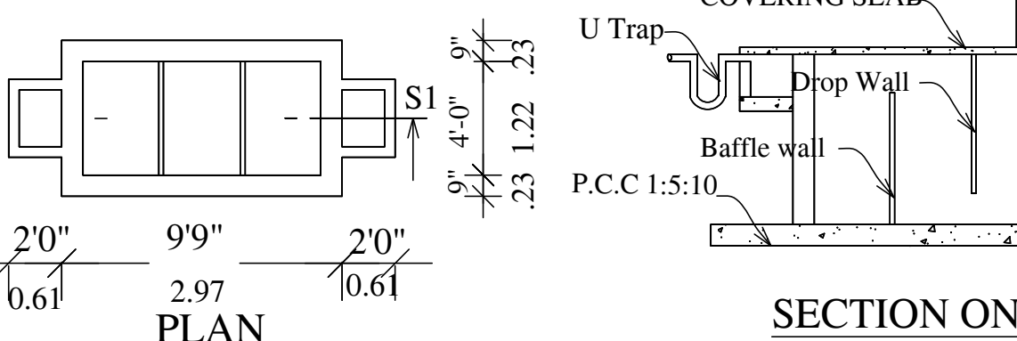
RAIN WATER HARVESTING TANK DETAIL
