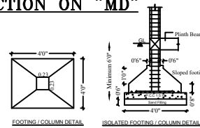
SECTION ON "MD"
