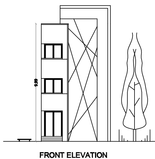
FRONT ELEVATION
