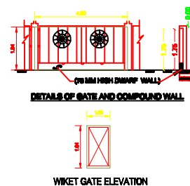
WIKET GATE ELEVATION
