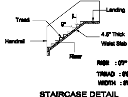
STAIRCASE DETAIL
