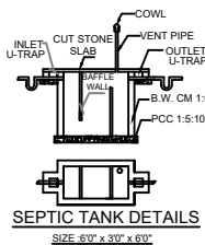
SEPTIC TANK DETAILS
