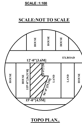
TOPO PLAN..
