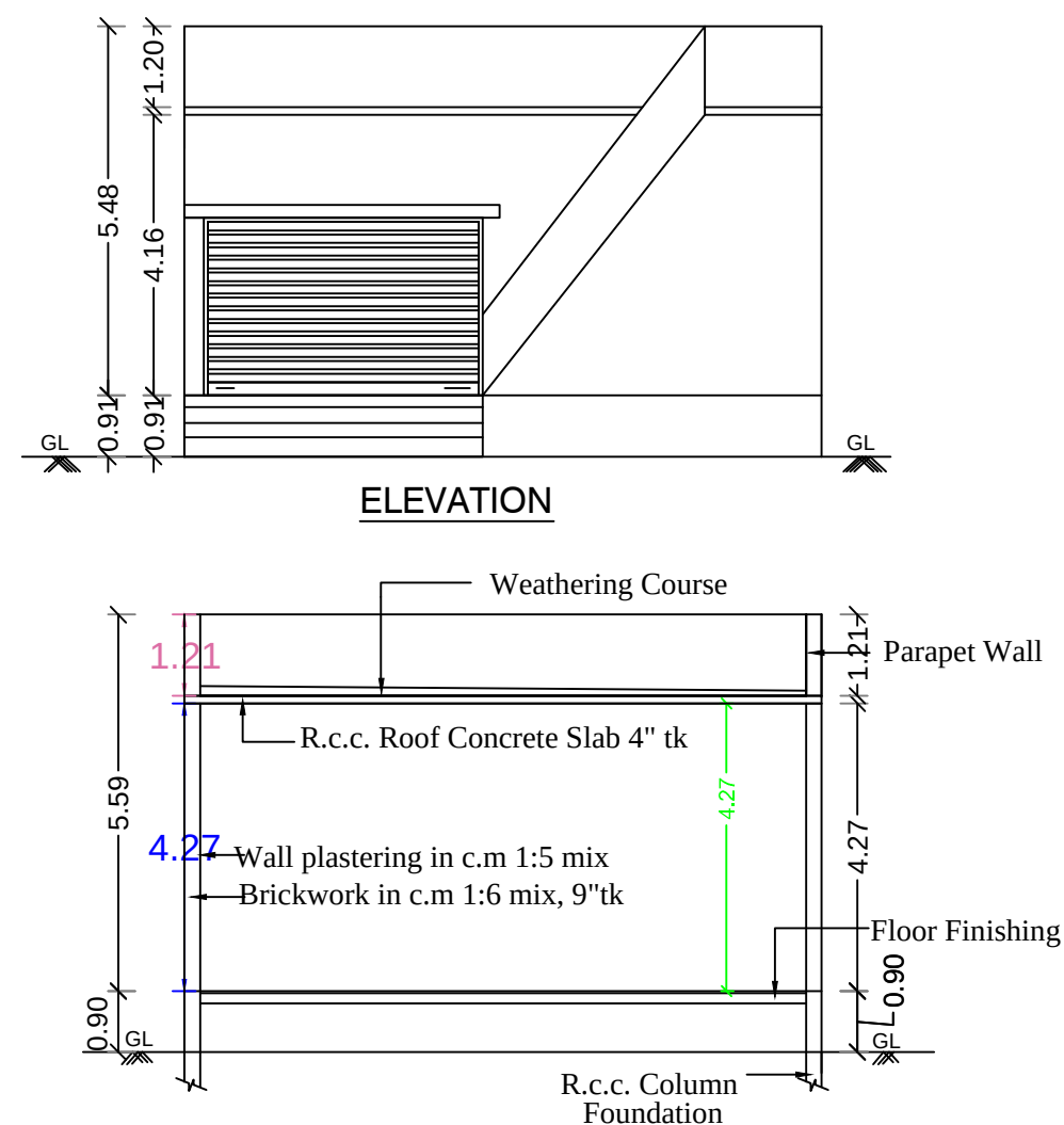
STAIR CASE DETAILS:-
