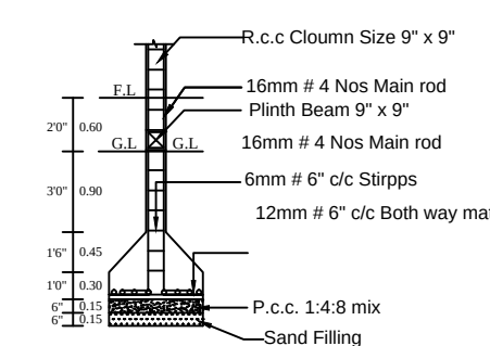
COLUMN DETIAL
