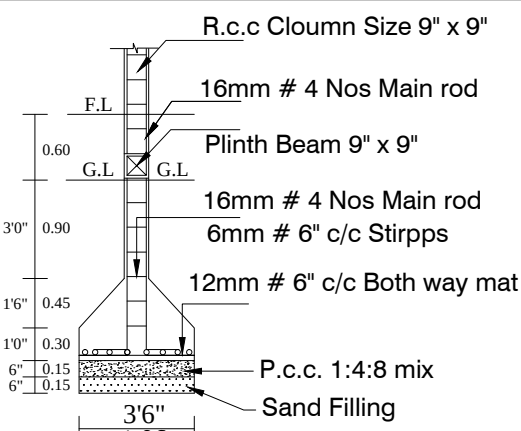
COLUMN DETIAL
