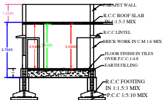
SECTION A B
