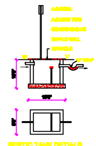
SEPTIC TANK DETAILS
