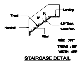
STAIRCASE DETAIL
