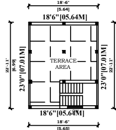
TERRACE FLOOR
