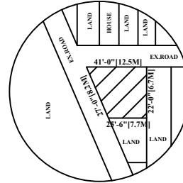
TOPO PLAN..
