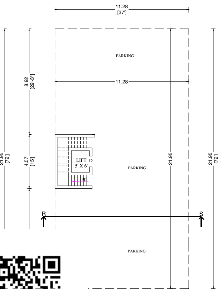
STILT FLOOR PLAN
