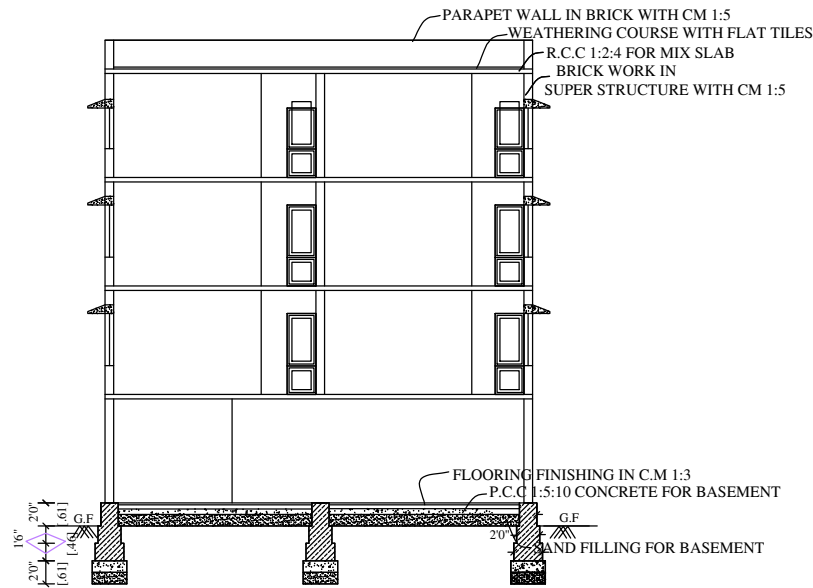
SECTION NO R-S
