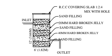
Waste Water Recycle Unit Not To Scale
