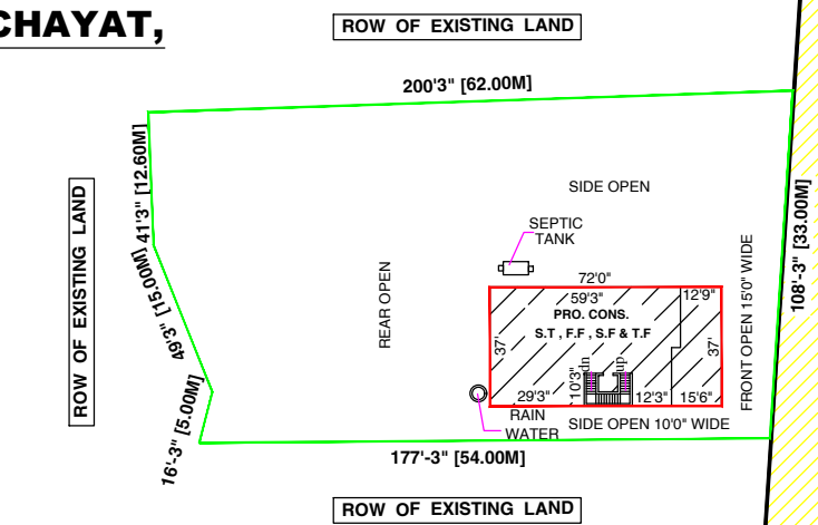
SITE PLAN SCALE - 1CM = 4M
