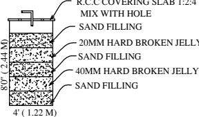
Rain Water Harvest Unit Not To Scale
