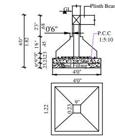
COLUMN DETAIL Not To Scale
