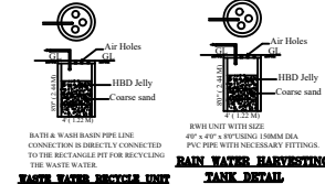
RAINWATER HARVESTING UNIT SIZE: 4'-0" X 4'-0" X 4'-0"
