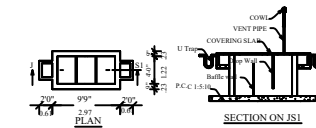
SECTION ON JS1
