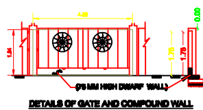
DETAILS OF GATE AND COMPOUND WALL WIKET GATE ELEVATION
