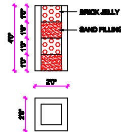
PERCOLATION PIT
