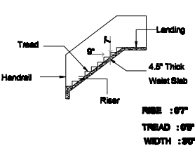
STAIRCASE DETAIL
