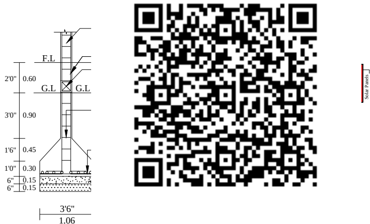
COLUMN DETAIL
