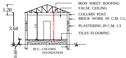
SECTION NN
