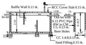
SEPTIC TANK & SOAK PIT
