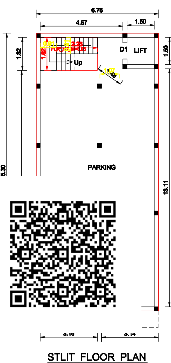
STLIT FLOOR PLAN
