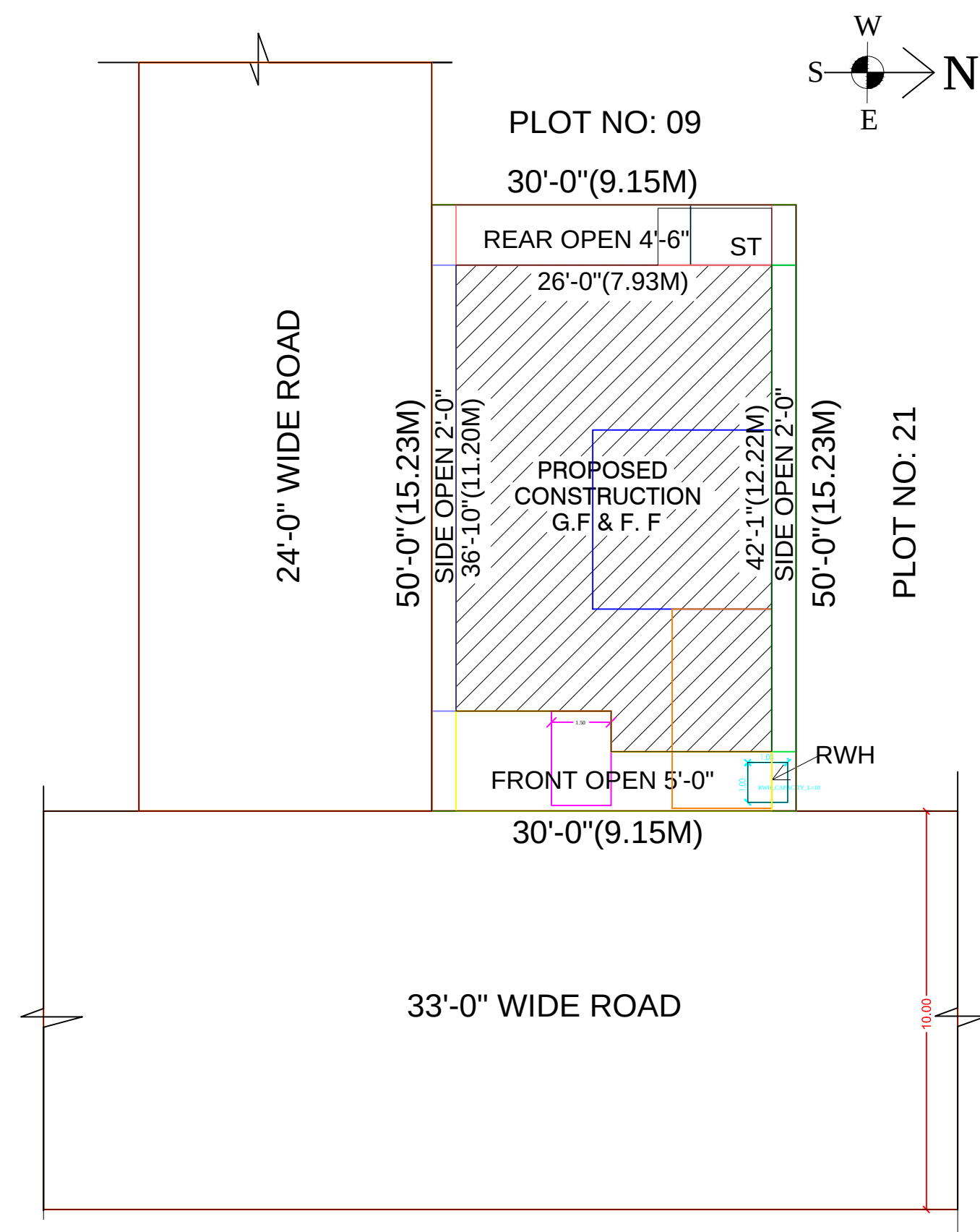
SITE PLAN SCALE: 1CM: 1M
