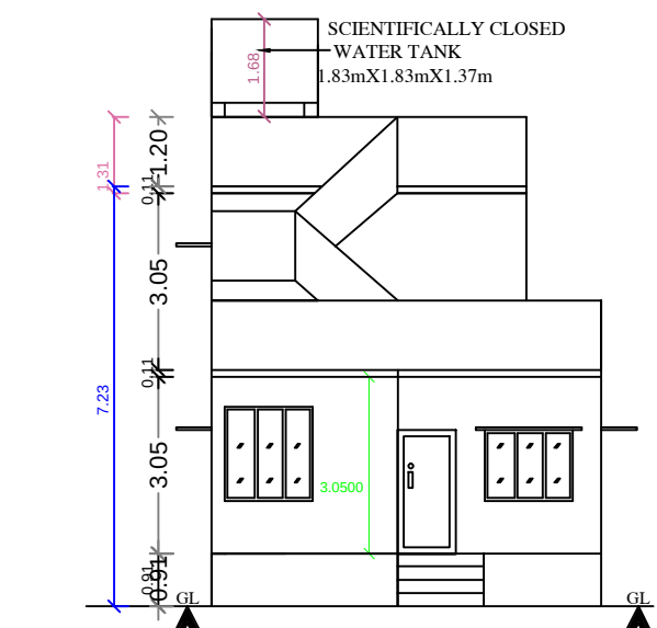
FRONT ELEVATION
