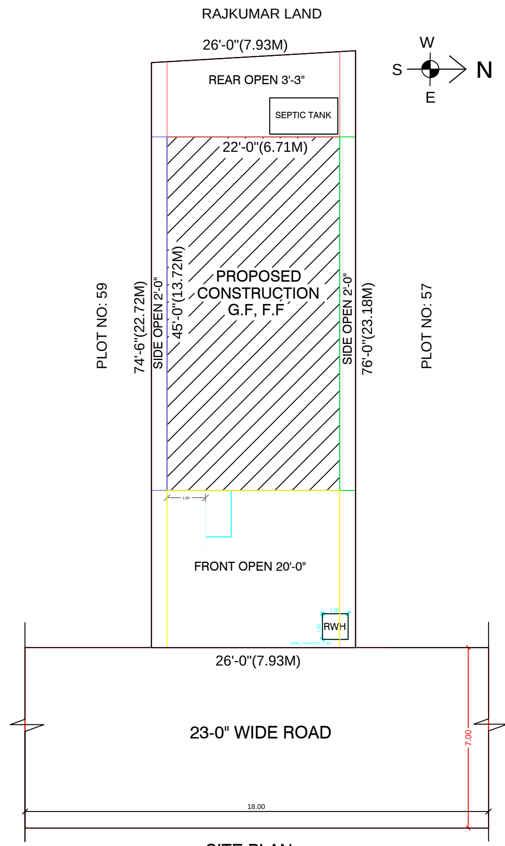
SITE PLAN (SCALE: 1CM : 1M)
