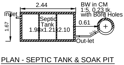
PLAN - SEPTIC TANK & SOAK PIT
