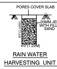
RAIN WATER HARVESTING UNIT
