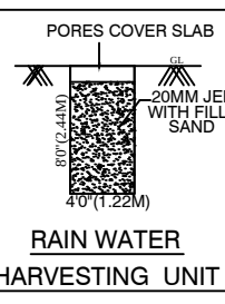
RAIN WATER HARVESTING UNIT
