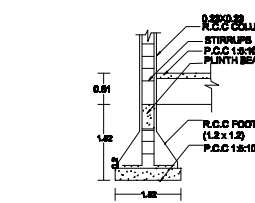
COLUMN DETAILS Size of column = 0.22m x 0.22m Not to scale
