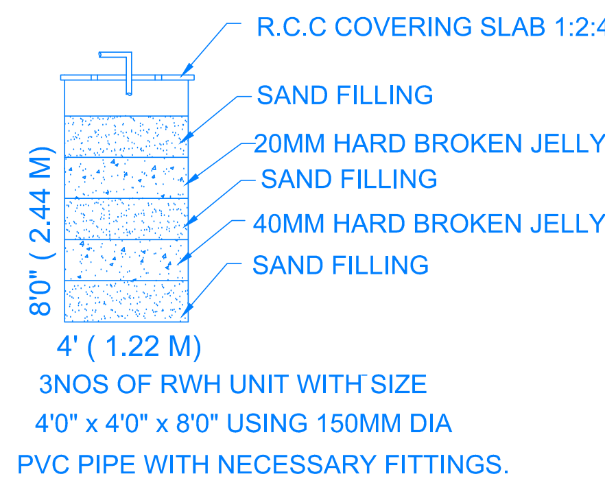
RAIN WATER HARVEST UNIT
