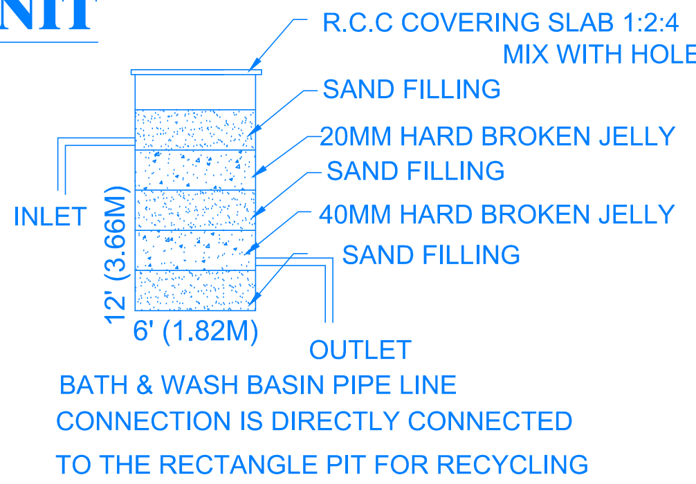
WASTE WATER RECYCLE UNIT
