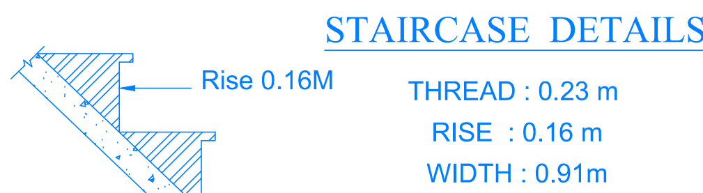
STAIRCASE DETAILS
