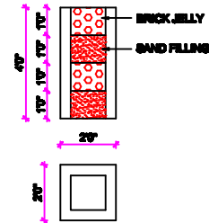
PERCULATION PIT
