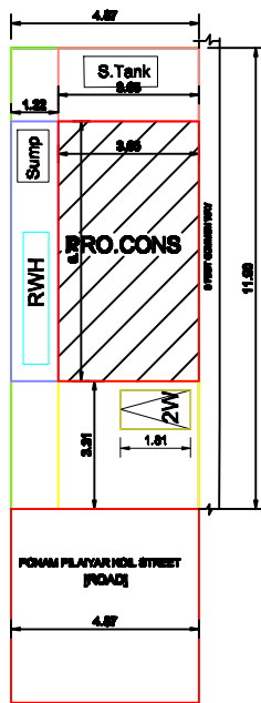
SITE PLAN
