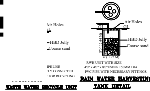
RAIN WATER HARVESTING UNIT SCALE: 1:50
