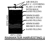
RAINWATER HARVESTING UNIT SIZE: 4'0" x 4'0" x 3'0" - 3'6"
