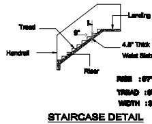
STAIRCASE DETAIL
