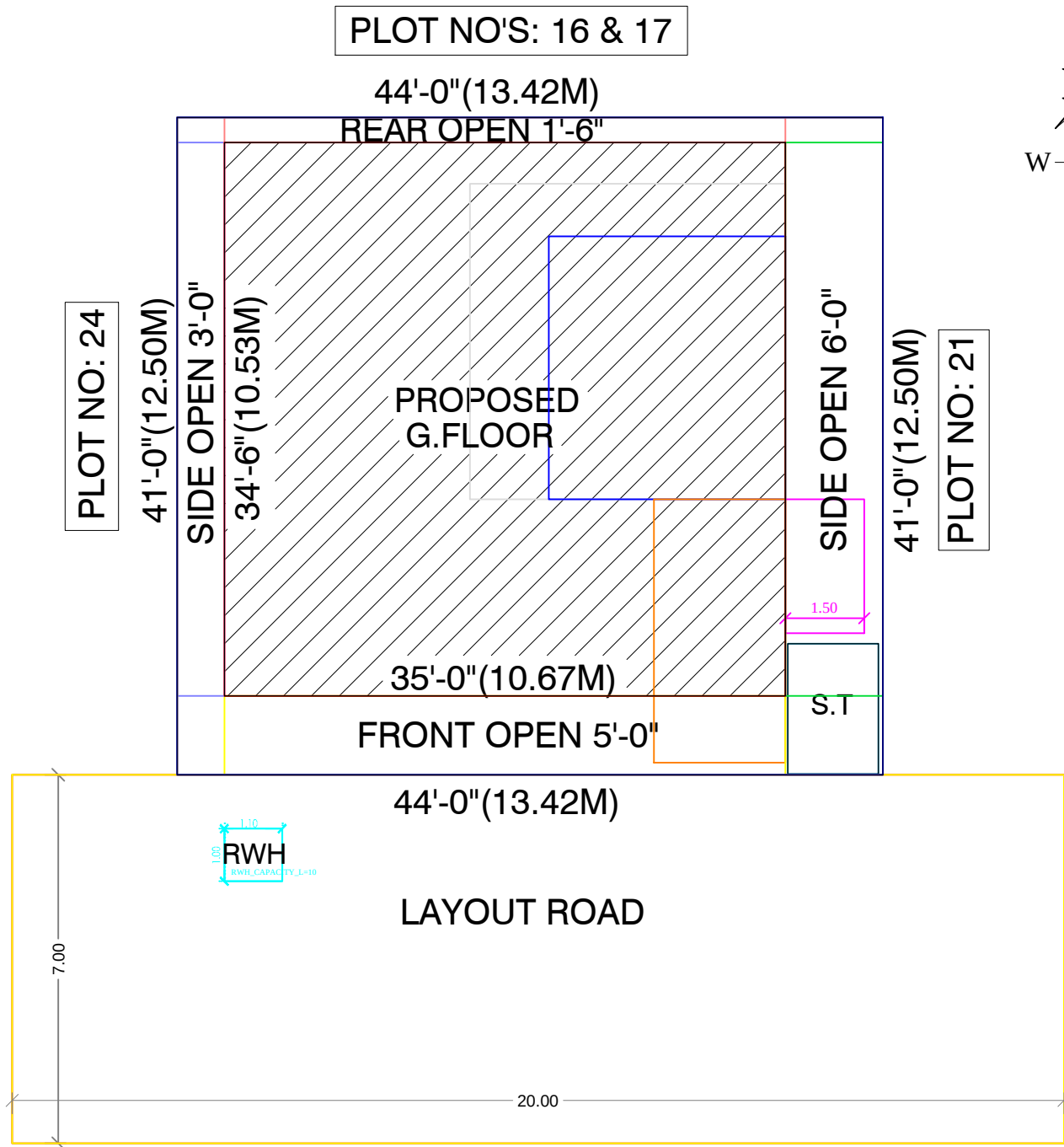
SITE PLAN SCALE: 1CM : 1M
