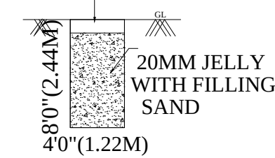
RAIN WATER HARVESTING UNIT
