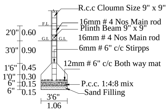
COLUMN DETIAL
