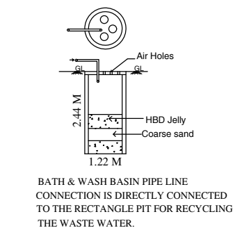
WASTE WATER RECYCLE UNIT
