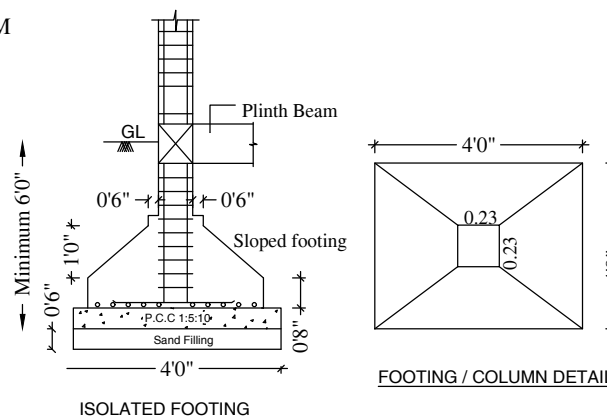
COLUMN DETAIL
