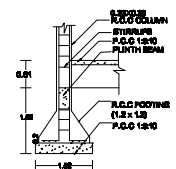
COLUMN DETAILS
