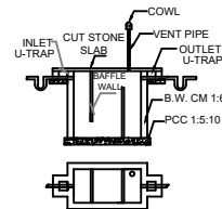
SEPTIC TANK DETAILS
