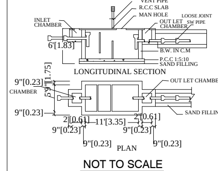
SEPTIC TANK:
