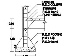
COLUMN DETAILS Size of column = 0.22m x 0.22m Not to scale
