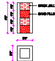
WATER TANK DETAIL
