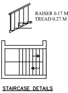
STAIRCASE DETAILS
