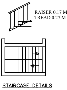
STAIRCASE DETAILS
