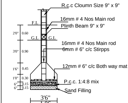
COLUMN DETIAL
