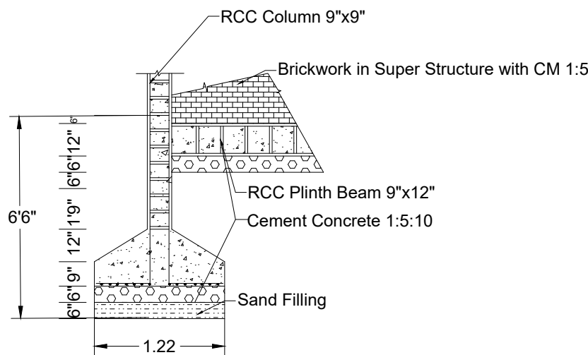
FOUNDATION DETAILS
