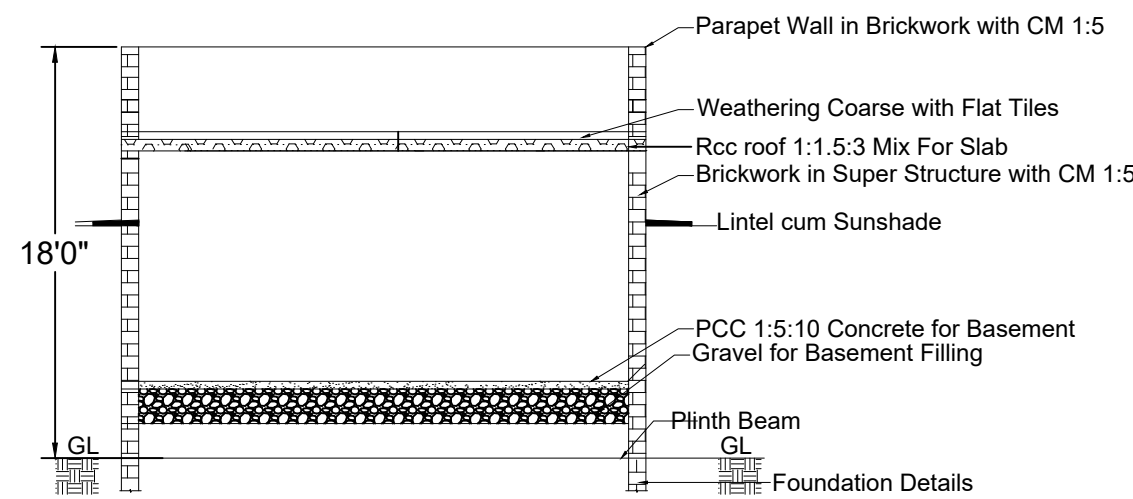
CROSS SECTION R-R
