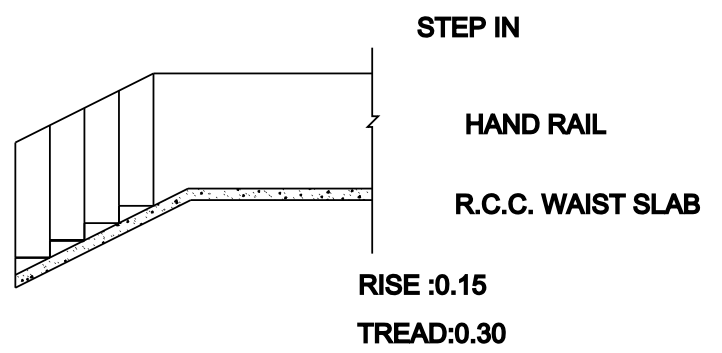
STAIR DETAILS
