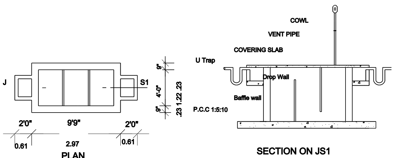
SEPTIC TANK DETAILS Using 'U' type trap 2 Nos in inlet, outlet & Vent pipe will be covered with Mosquito proof covering net in inner side and top of vent pipe.
