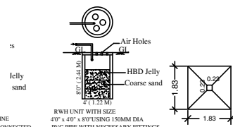
SECTION ON JS1
