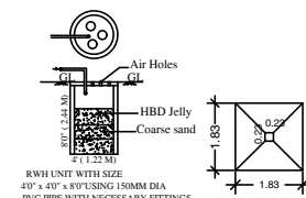
RAIN WATER HARVESTING TANK DETAIL
