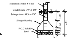
ISOLATED FOOTING / COLUMN DETAIL
