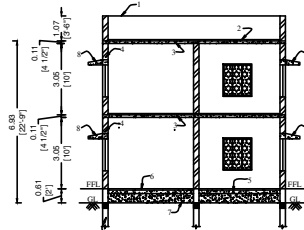
SECTION ON "JS"
