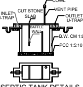
SEPTIC TANK DETAILS SIZE: 40' x 30' x 60'
