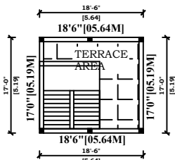
TERRACE FLOOR
