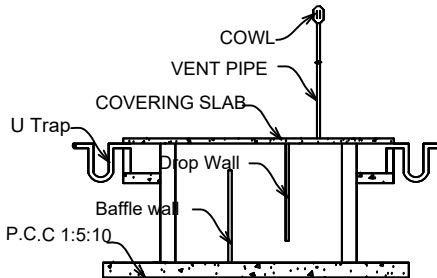
SECTION ON AB1
