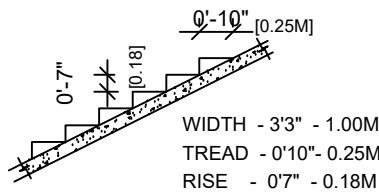
STAIRCASE DETAILS
