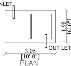
SEPTIC TANK
