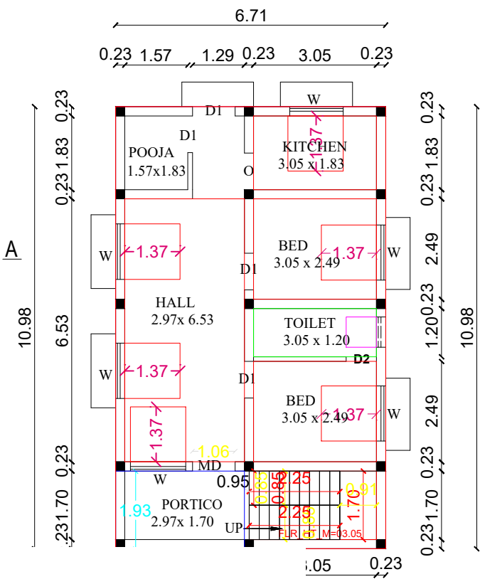
FLOOR PLAN 100
