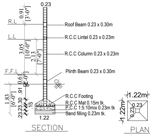
R.C.C FOUNDATION AND COLUMN DETAILS
