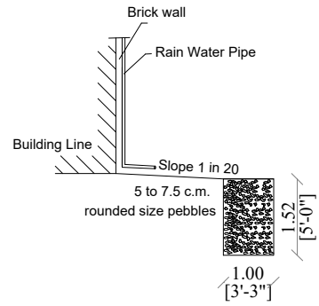
PERCOLATION PIT
