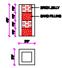
PERCOLATION P.T.
