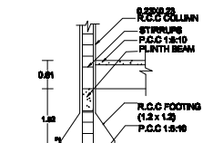
COLUMN DETAILS Size of column = 0.23m x 0.23m Not to scale
