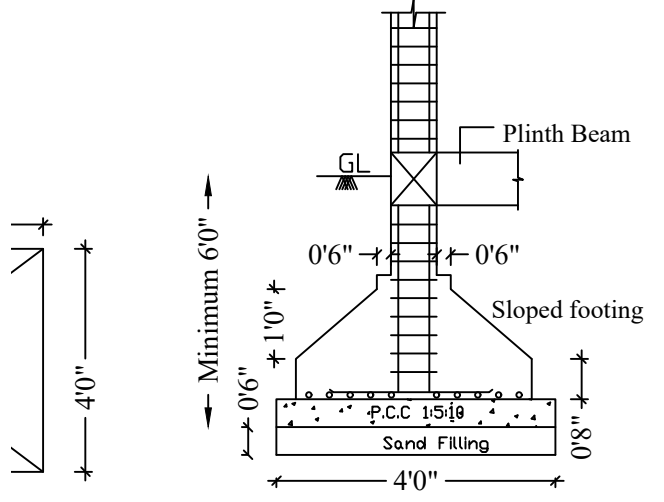
ISOLATED FOOTING / COLUMN DETAIL
