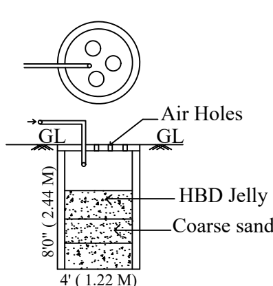
RAIN WATER HARVESTING TANK DETAIL
