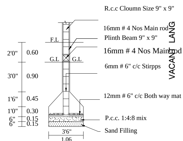
COLUMN DETIAL
