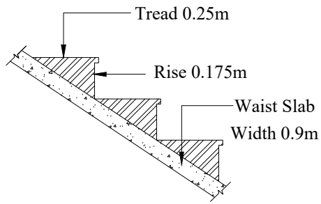
SECTION FOR STAIRCASE (NOT TO SCALE)
