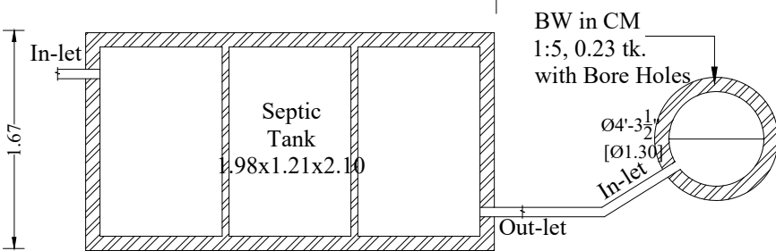
SEPTIC TANK PLAN & SOAK PIT PLAN (NOT TO SCALE)
