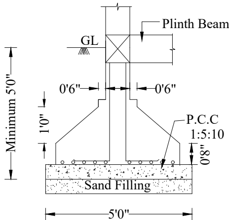
ISOLATED FOOTING (5'-0"x5'-0") (NOT TO SCALE)
